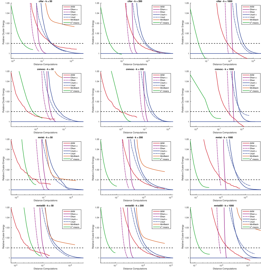
Figure 3: Cluster Energy (relative to best Lloyd++ energy) vs distance computations on cifar, cnvoc, mnist and mnist50 for k \in \{50, 200, 1000\} . For AKM and k^2 -means, we use the parameter with the highest algorithmic speedup at 1% error.
