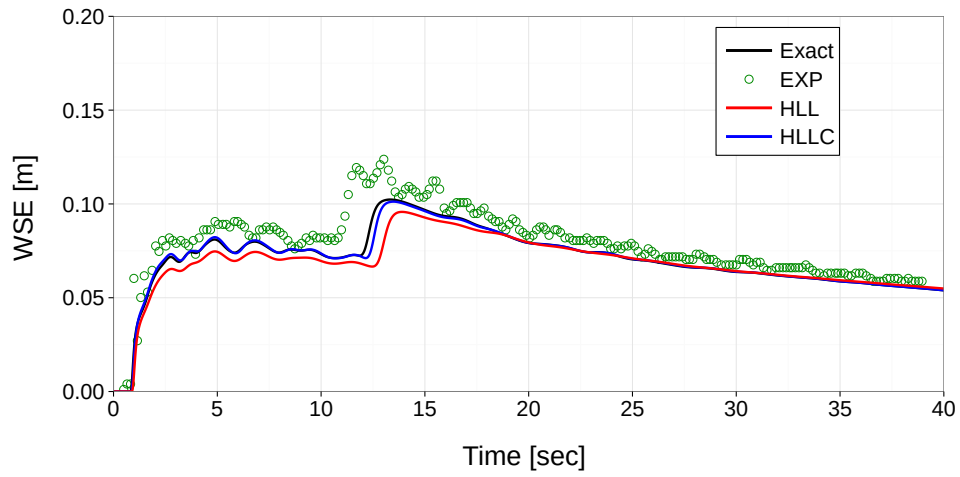
Figure 1.36 H_BP_3 : Water surface elevation at G3
